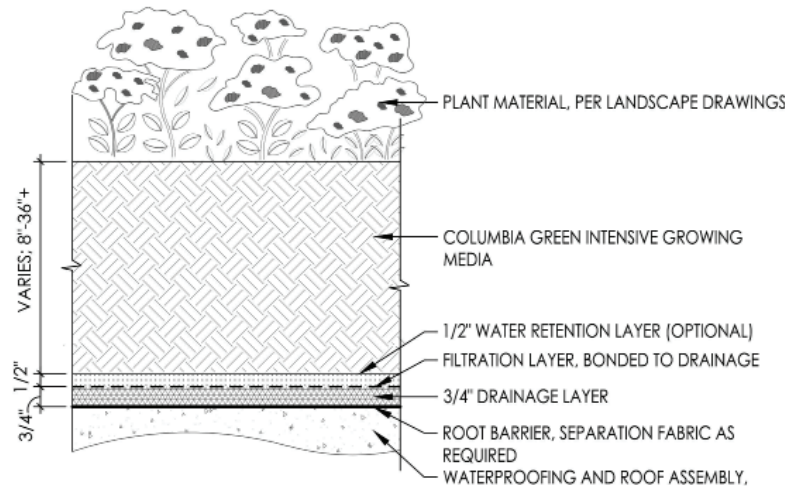
TYPICAL PLANTER INTERIOR DETAIL
