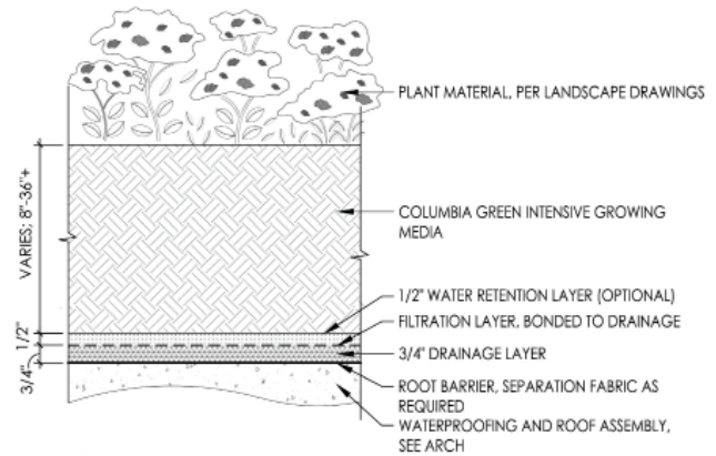
TYPICAL AMENITY DECK DETAIL
